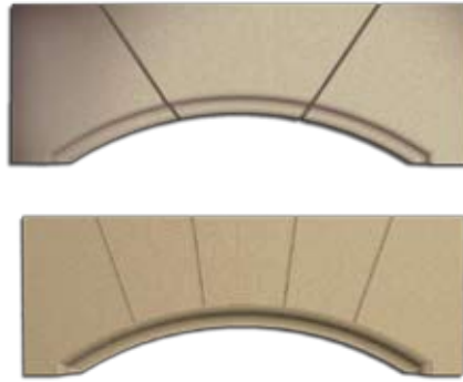
SPLAYED DETAIL OPTIONS
