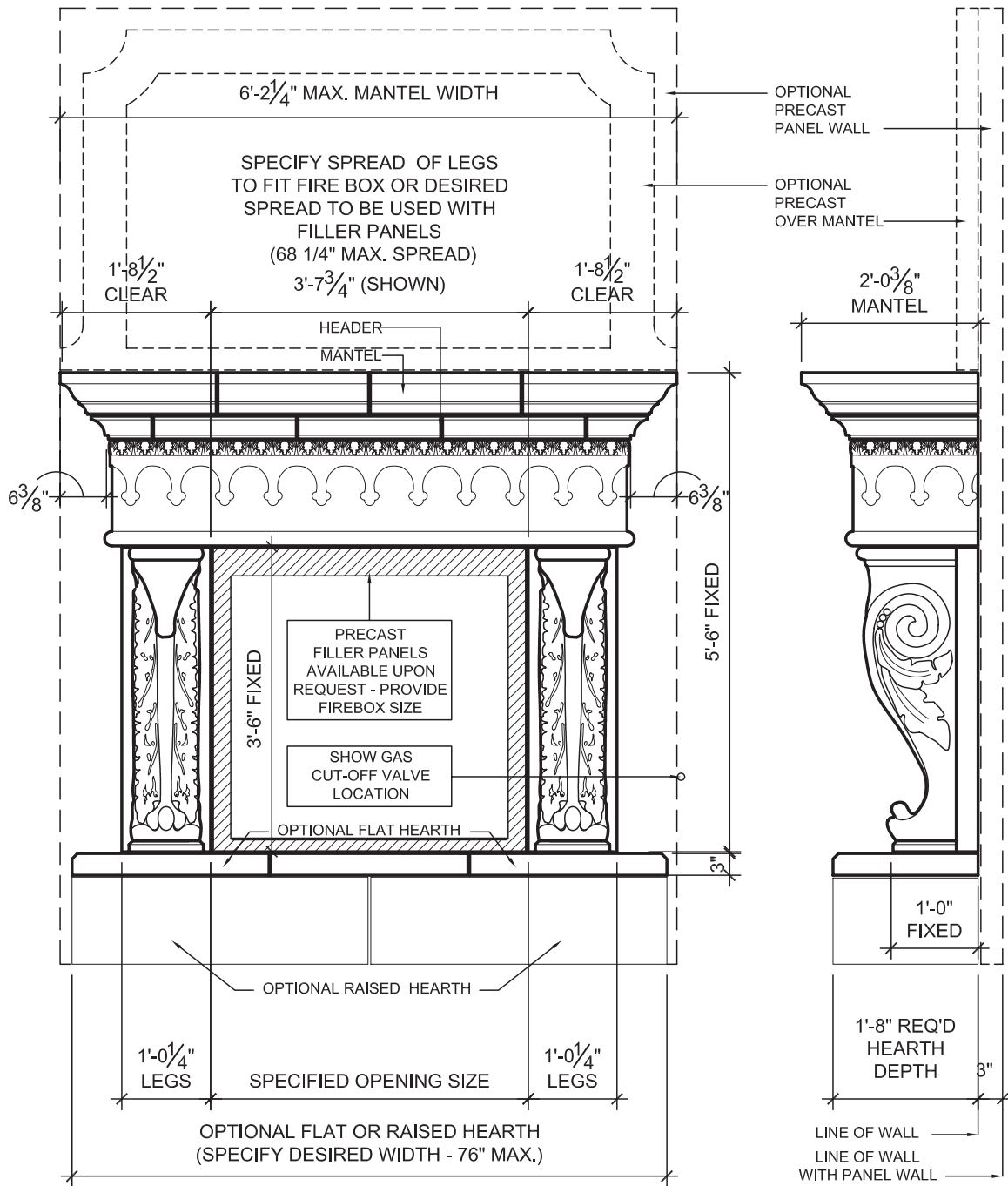
A ELEVATION - BELAVERA FIREPLACE 1/2" = 1'-0"
