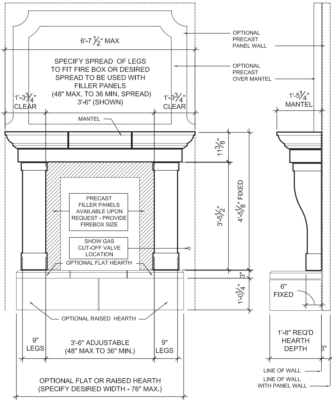
A ELEVATION - BERKLEY 1/2" = 1'-0"
